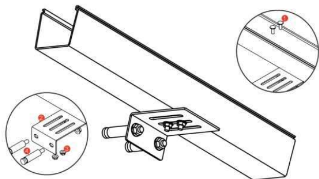
60X60 WALL MOUNTING
