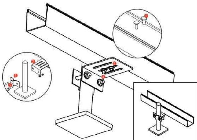
60X60 UNDER ACCESS FLOOR MOUNTING
