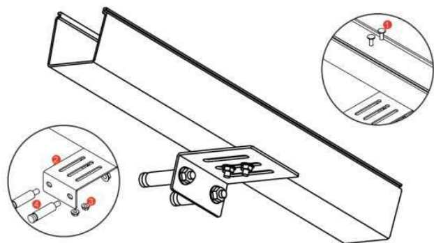
60X60 WALL MOUNTING
